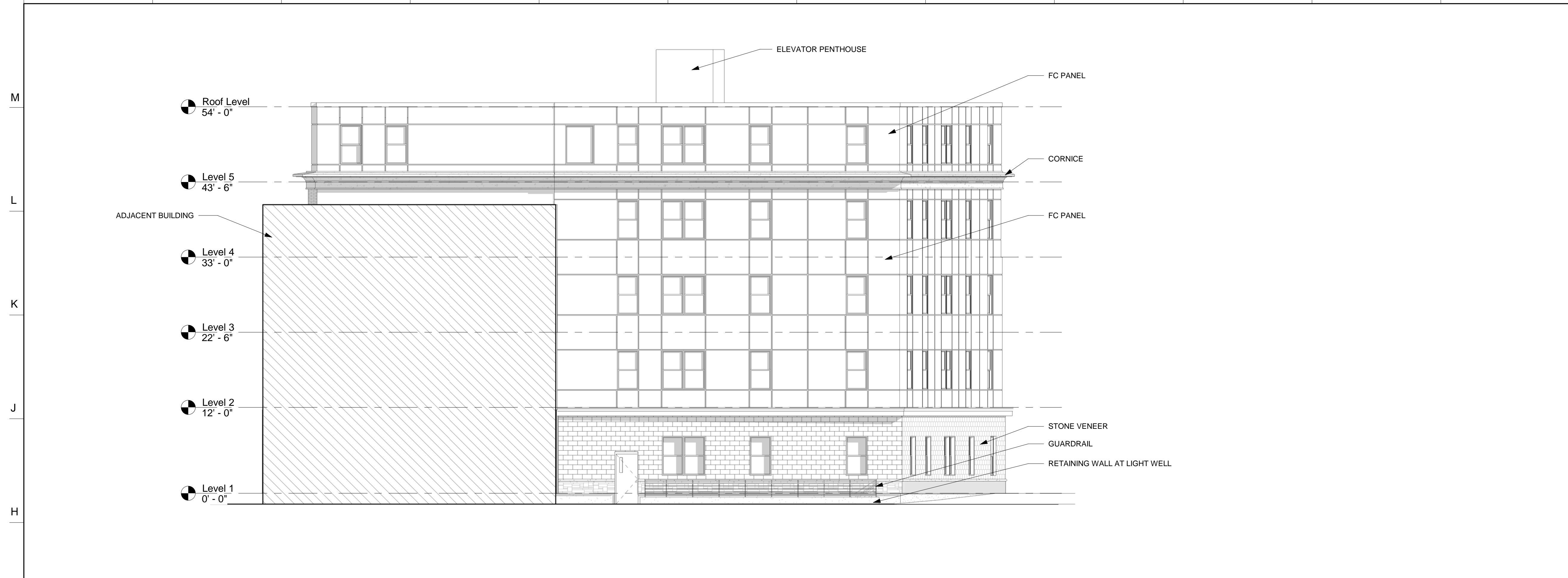
G-1 RIGHT ELEVATION (NORTHWEST) 1/8" = 1'-0"
