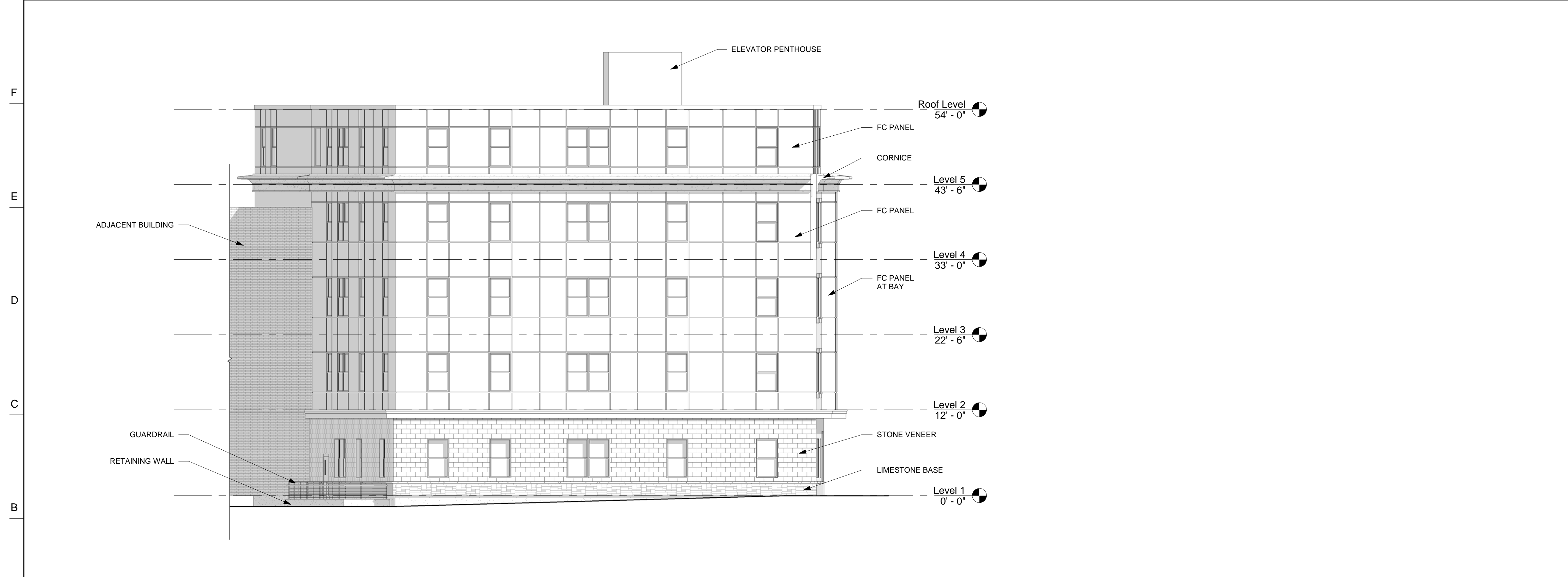
A-1 BACK ELEVATION (SOUTHWEST) 1/8" = 1'-0"
