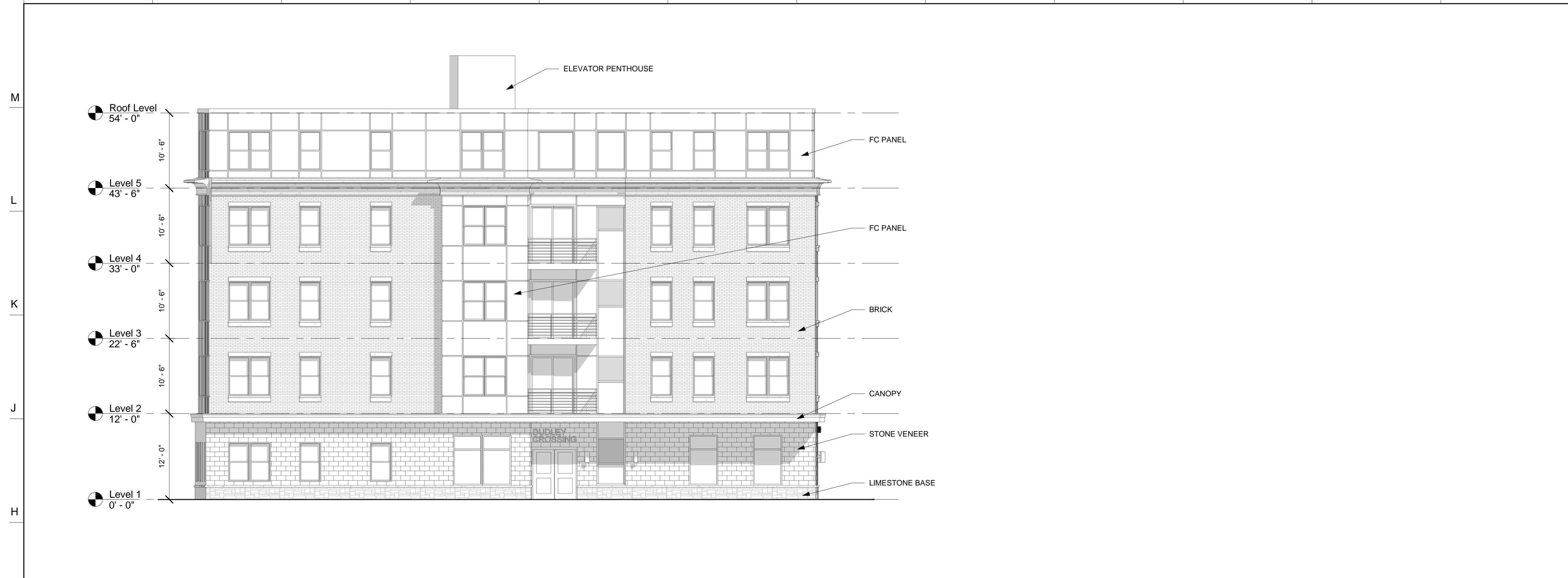
G-1 LEFT ELEVATION (SOUTHEAST) 1/8" = 1'-0"
