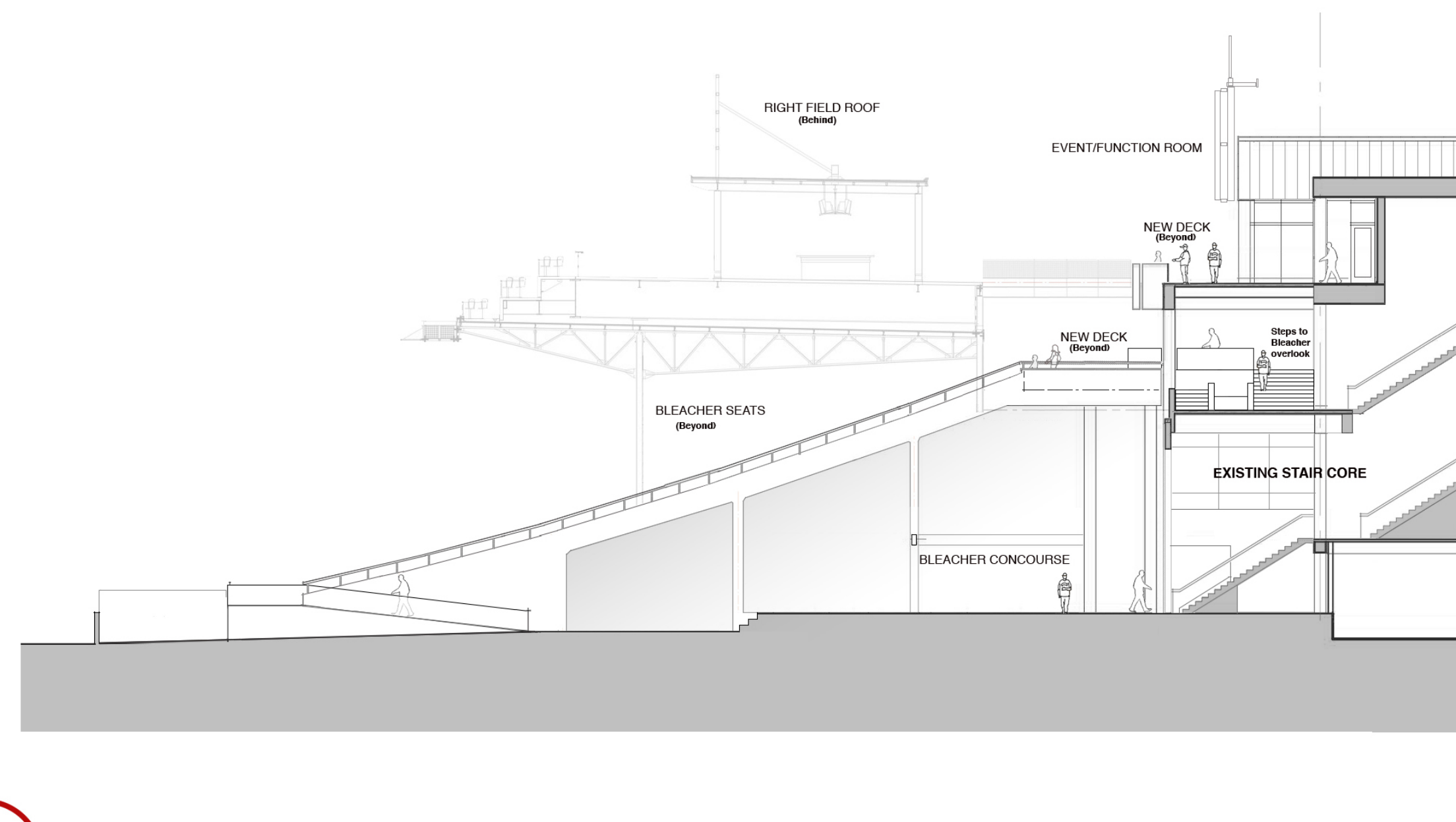
2 SECTION THRU STAIR CORE
