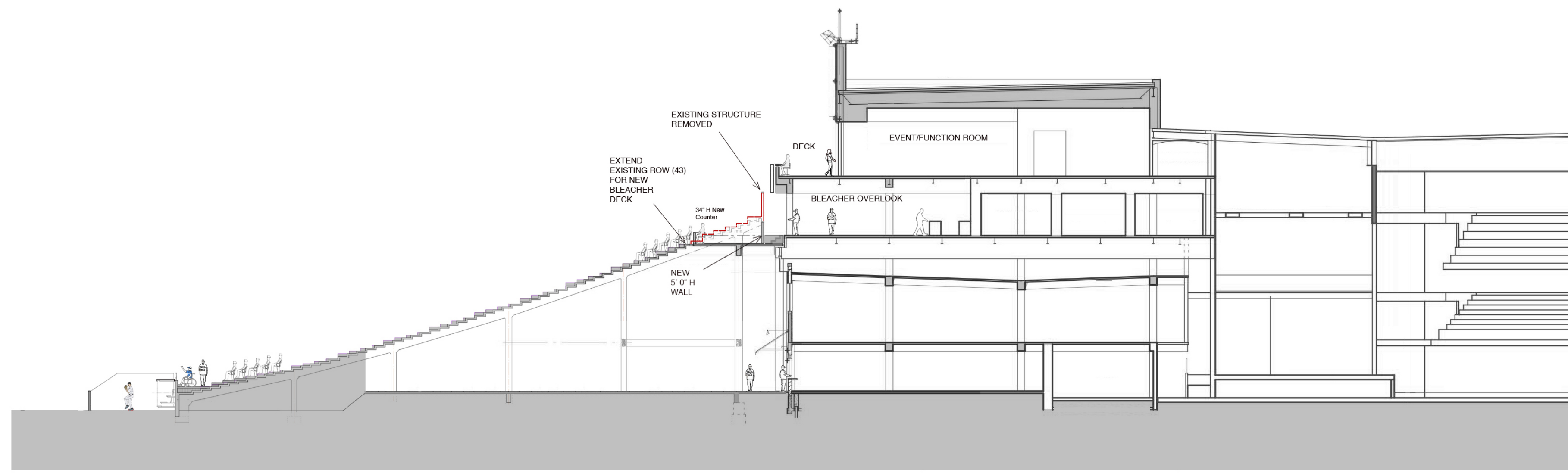
1 SECTION THRU BLEACHER CONCOURSE
