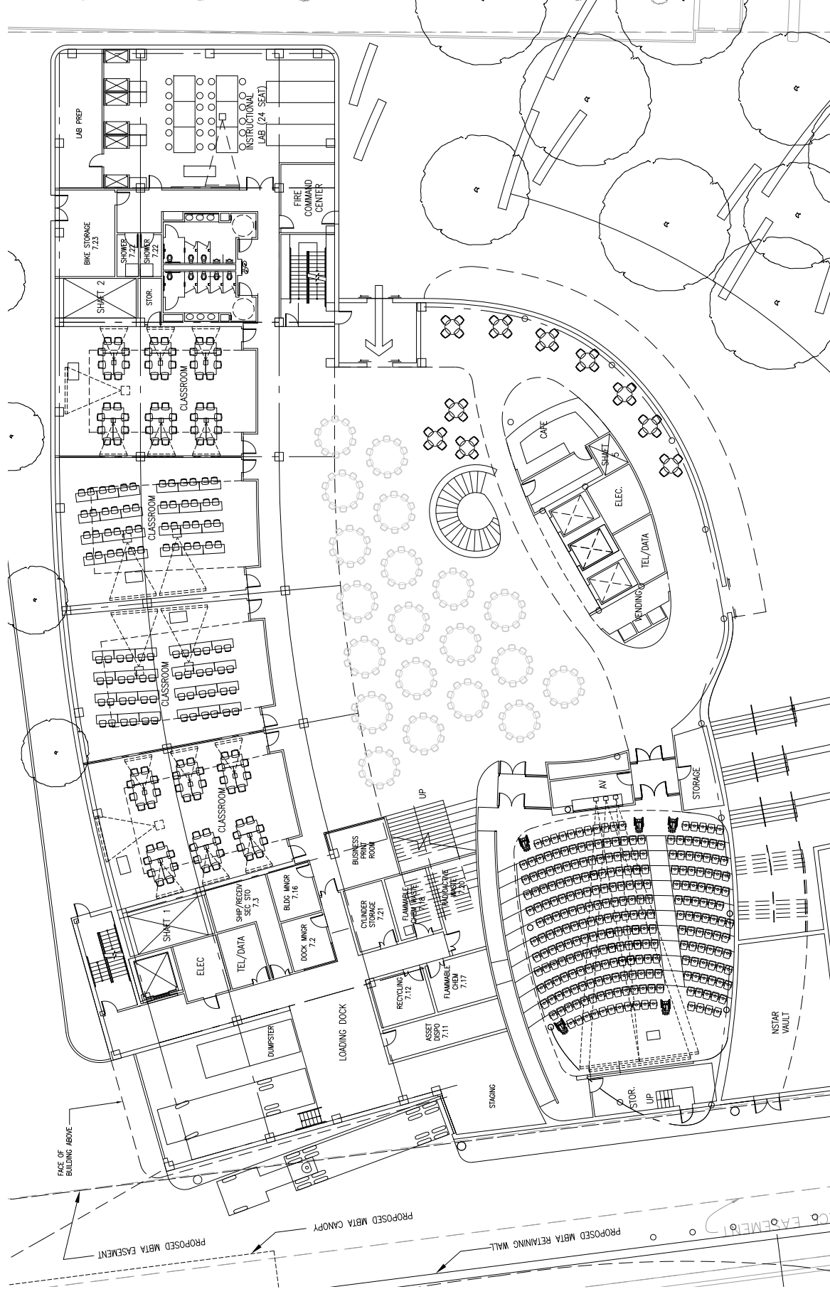
Figure 3-11. Level One Plan - Teaching / Bldg Support Scale: 1/32" = 1'-0"
