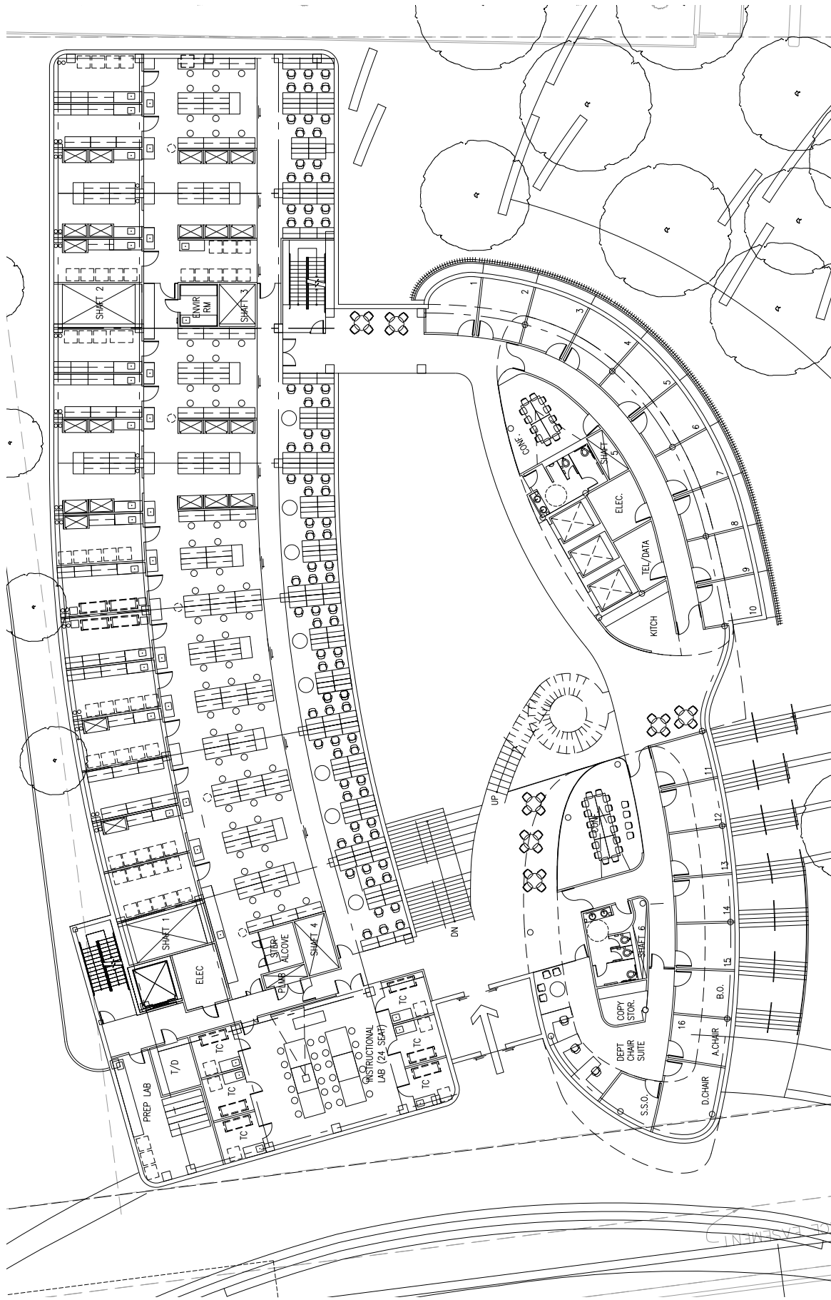
Figure 3-12. Level Two Plan - Admin / Teaching / Research Scale: 1/32" = 1'-0"
