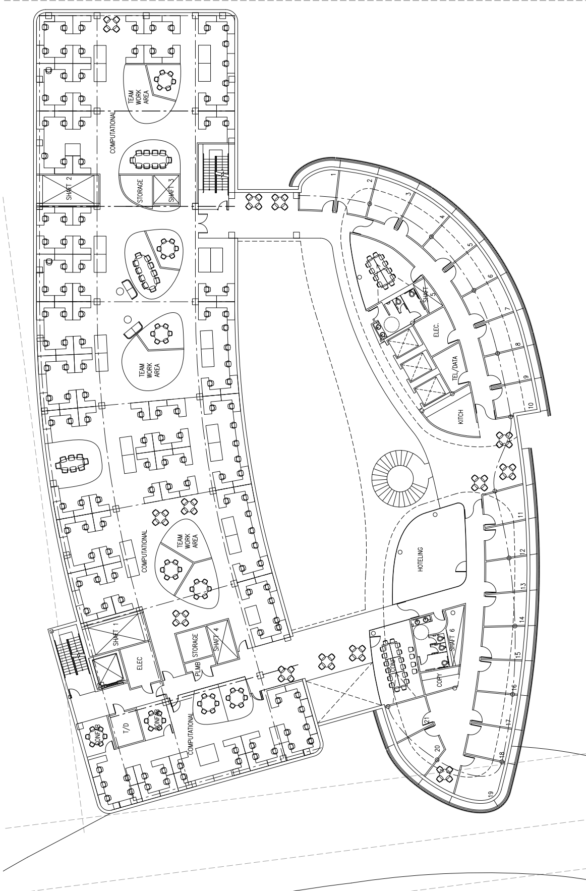
Figure 3-16. Level Six Plan - Research Scale: 1/32" = 1'-0"
