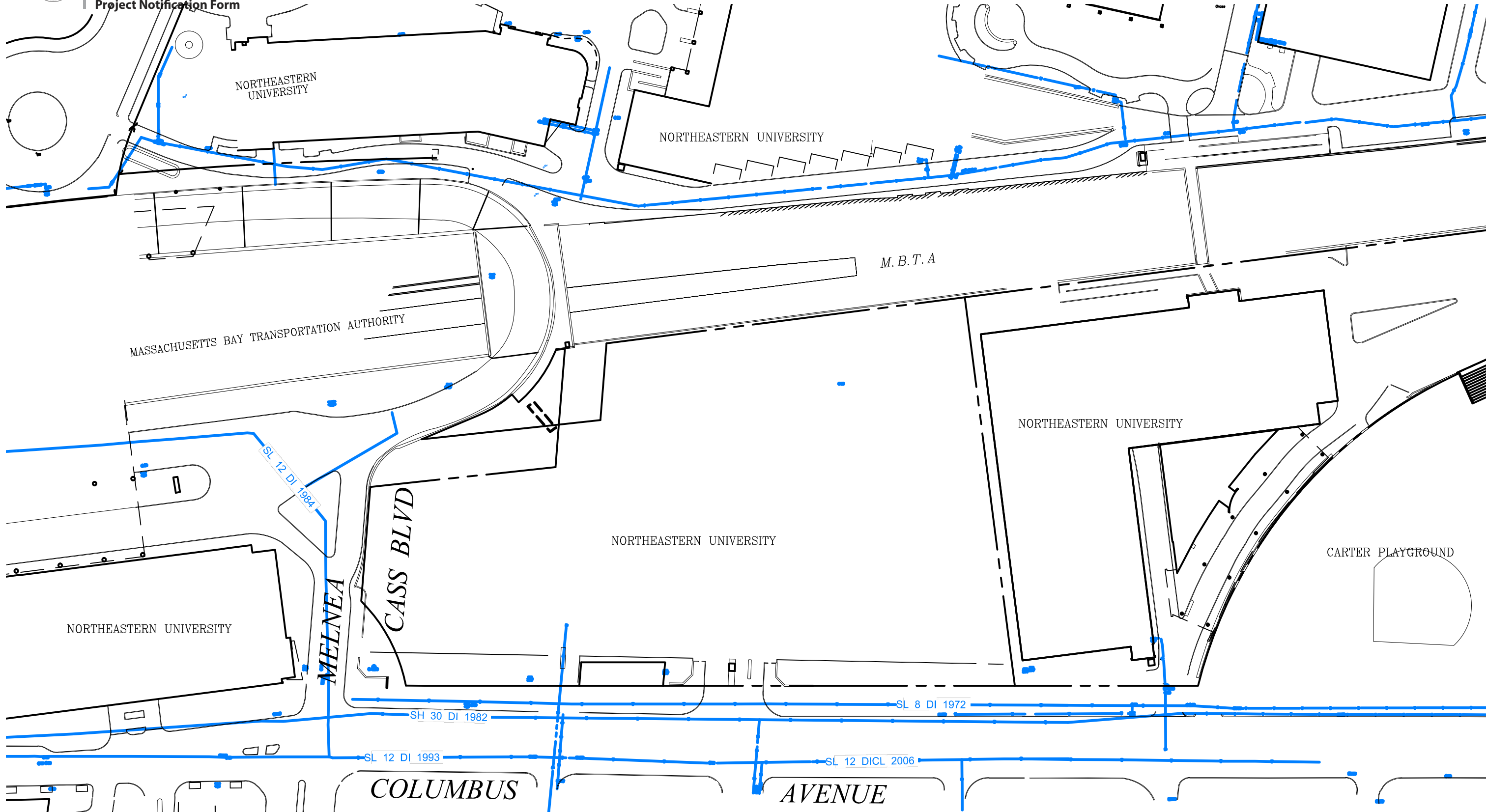
Figure 6-2 Existing Water Utility Infrastructure
