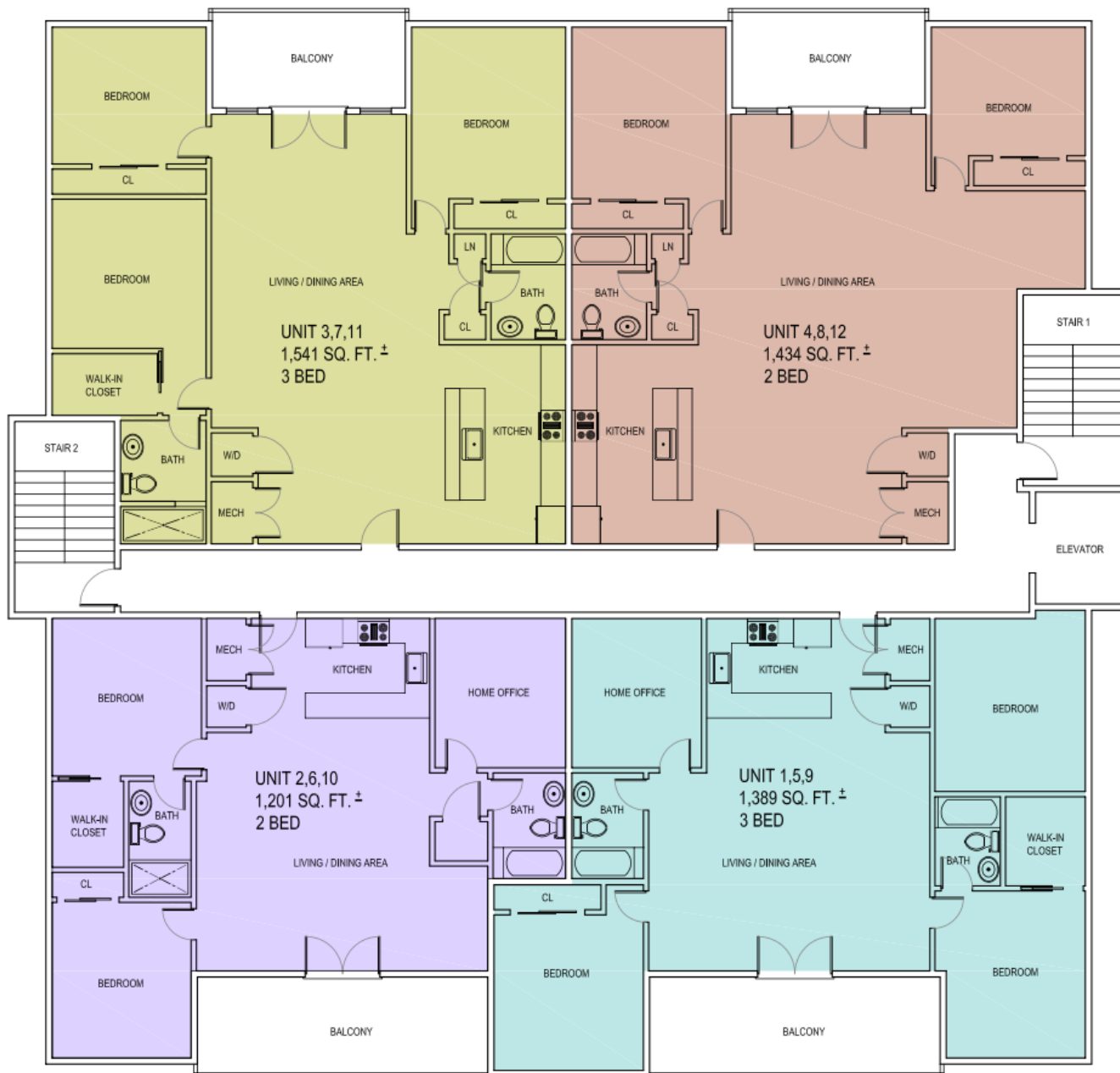
SECOND, THIRD & FOURTH FLOOR PLANS
