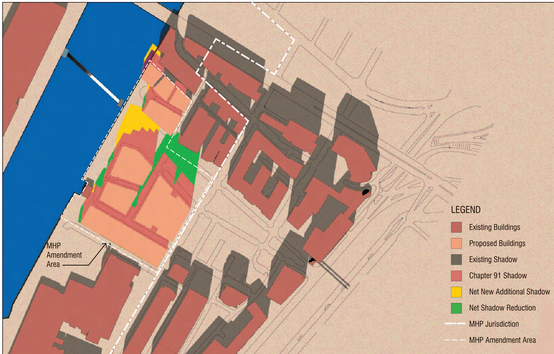
Figure A2-5 Shadow Studies: 1PM, October 23
