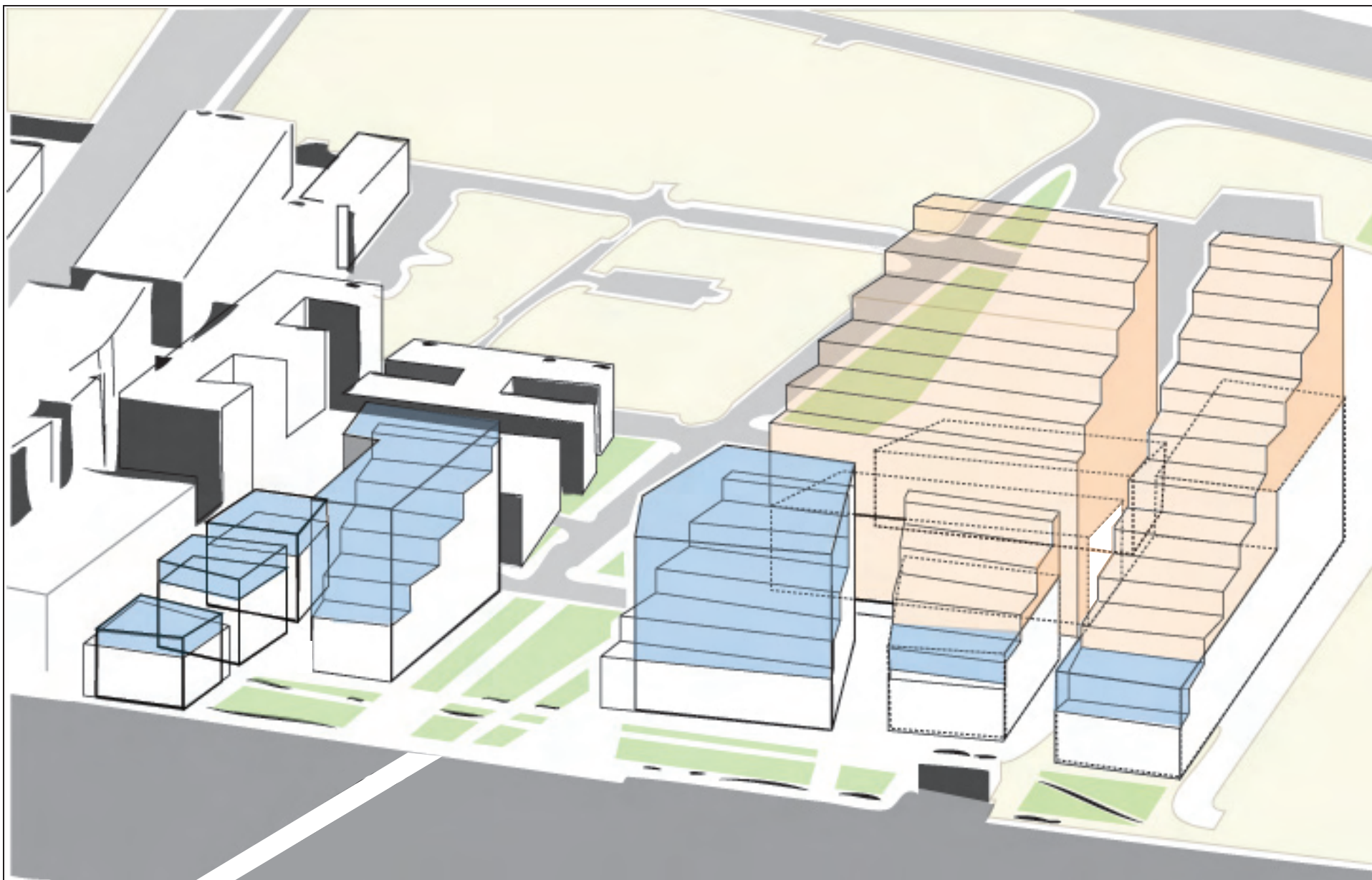
Figure 6-6 Chapter 91 with Proposed Buildable Volume
